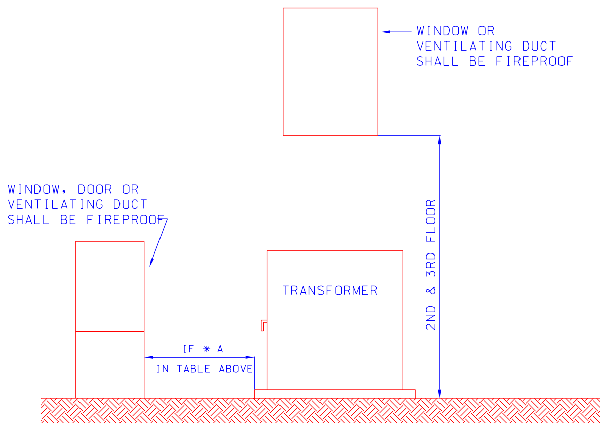
ELEVATION VIEW
