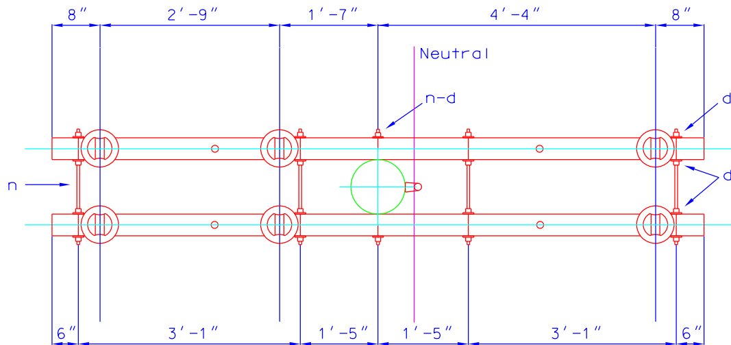
PLAN
