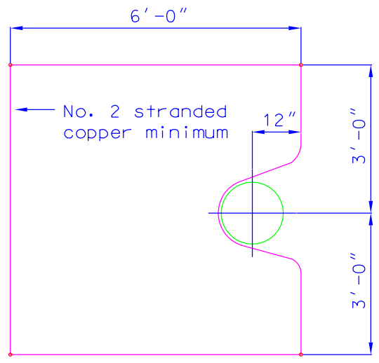
SECTION X-X (Detail of ground grid)
